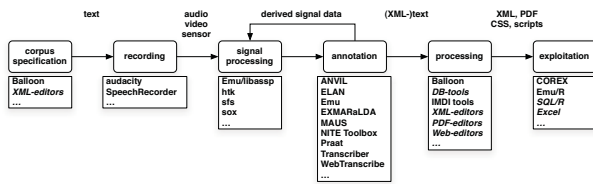
Figure 2: Speech database creation and exploitation workflow and a selection of tools used in the individual tasks.
