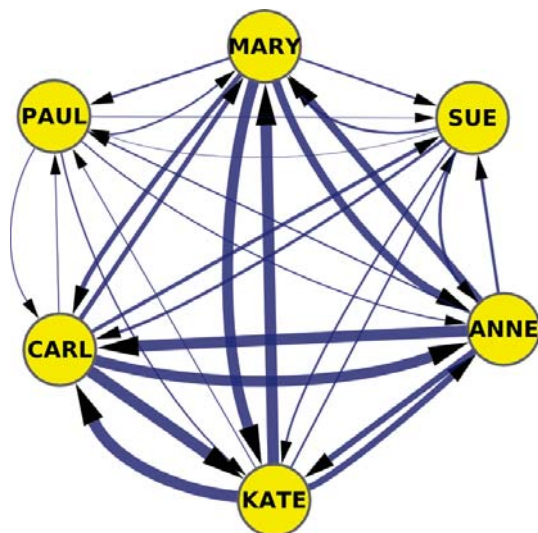
Figure 2: Speaker interaction
