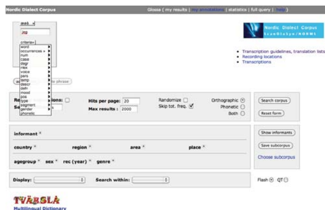
Figure 4: The search window
