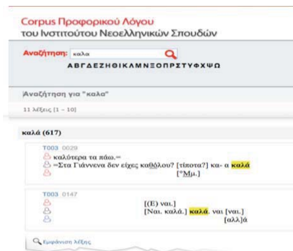
Figure 2: Search results
