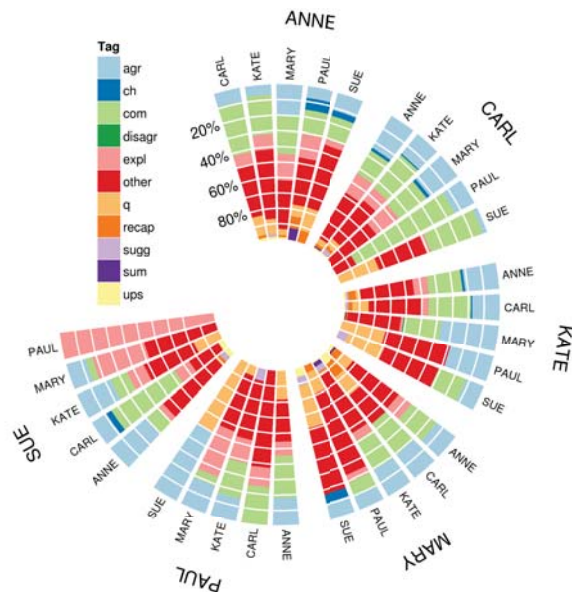
Figure 3: Speaker-Tag distribution
