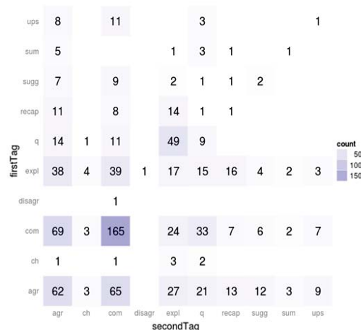
Figure 4: Tag pattern
